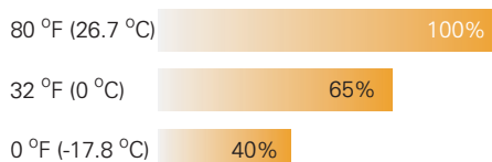
Comparison of short term power available from a fully charged battery at various temperatures
